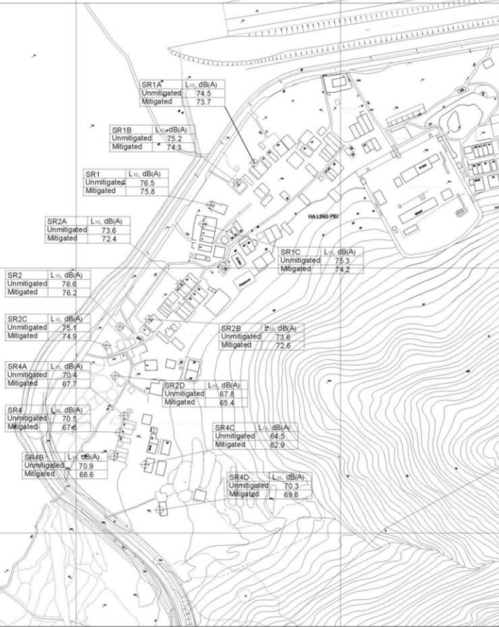
Maximum Unmitigated and Mitigated Operational Noise Levels at Representative NSR
